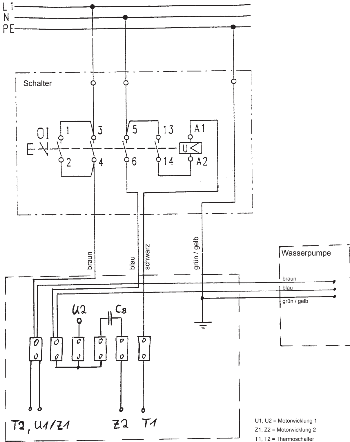
CTS•56, Elektro-Schaltplan, 230 V
